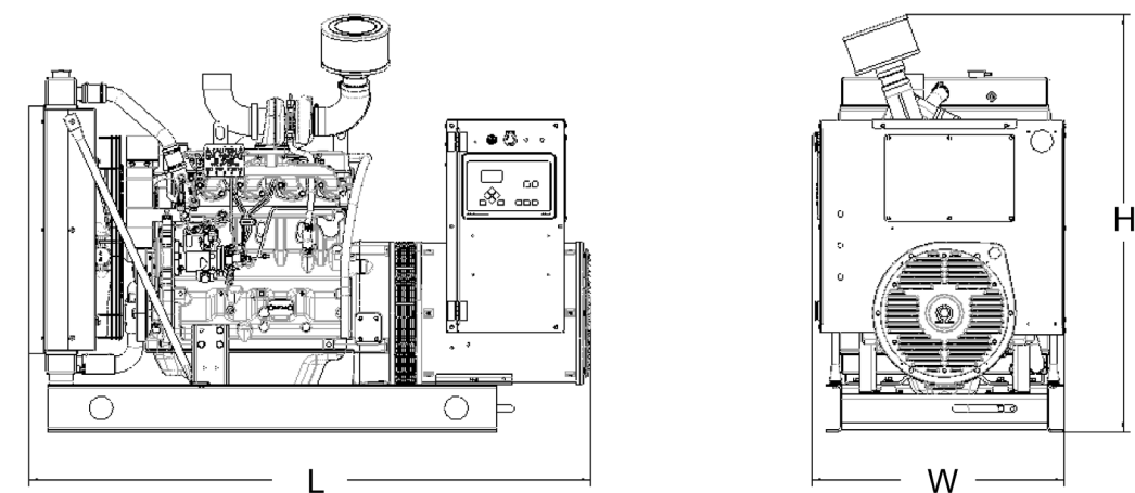
Drawing above for illustration purposes only, based on standard open power 480 volt generator set. Lengths may vary with other voltages. Do not use for installation design. See website for unit specific template drawings.
