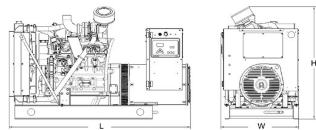
Drawing above for illustration purposes only, based on standard open power 480 volt generator set. Lengths may vary with other voltages. Do not use for installation design. See website for unit specific template drawings.
