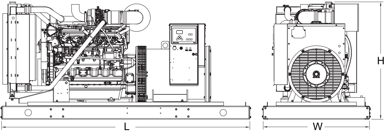
Drawing above for illustration purposes only, based on standard open power 480 volt generator set. Lengths may vary with other voltages. Do not use for installation design. See website for unit specific template drawings.
